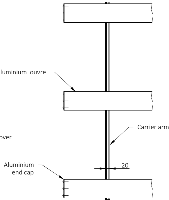
Elevation Detail
