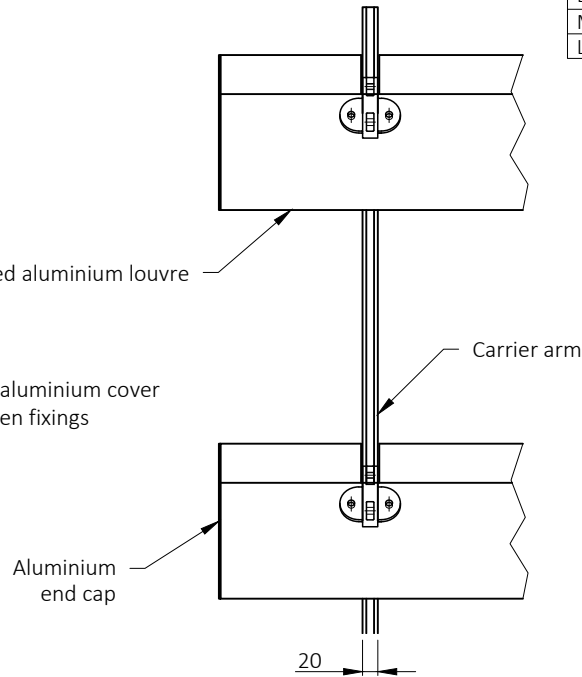
Elevation Detail
